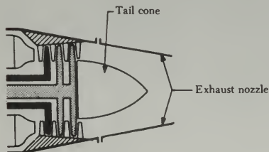
FIGURE 2-34. Conventional convergent exhaust duct.
